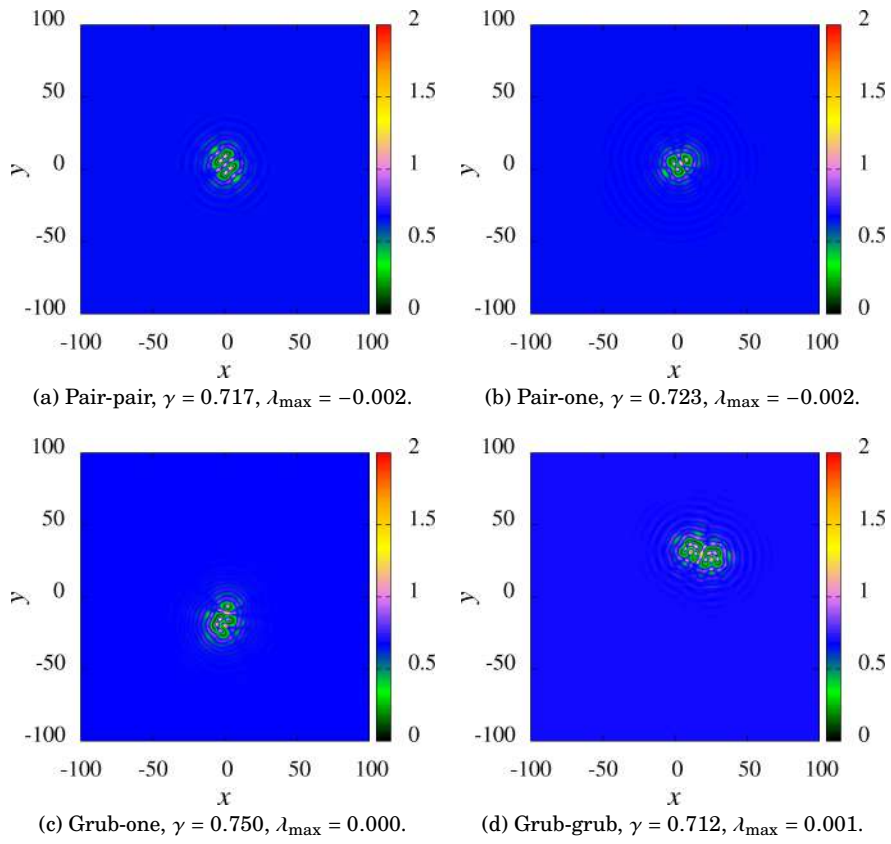
Fig. 4.— Localized clusters of simple patterns.
