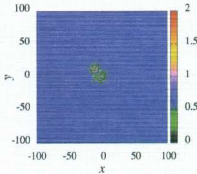
(c) Pentagon-grub, \gamma = 0.730 , \lambda_{\max} = -0.001 .
