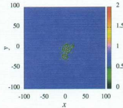
(b) Pentagon-circular-one, \gamma = 0.758 , \lambda_{\max} = 0.015 .
