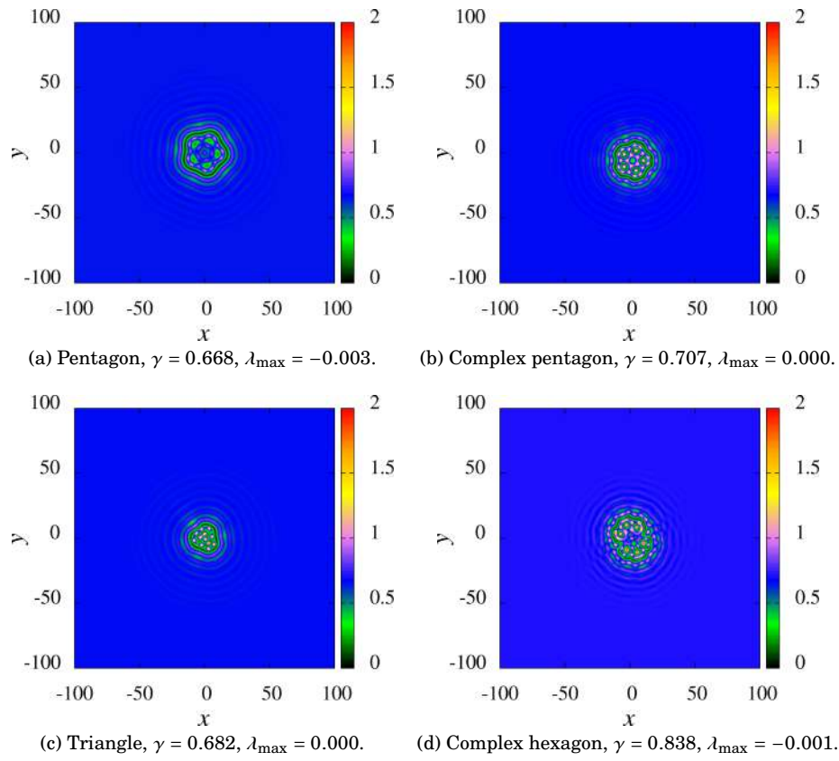
Fig. 2.— Localized regular patterns.
