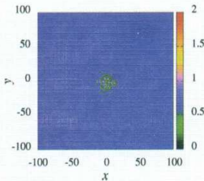
(a) Stadium-one, \gamma = 0.732 , \lambda_{\max} = 0.010 .
